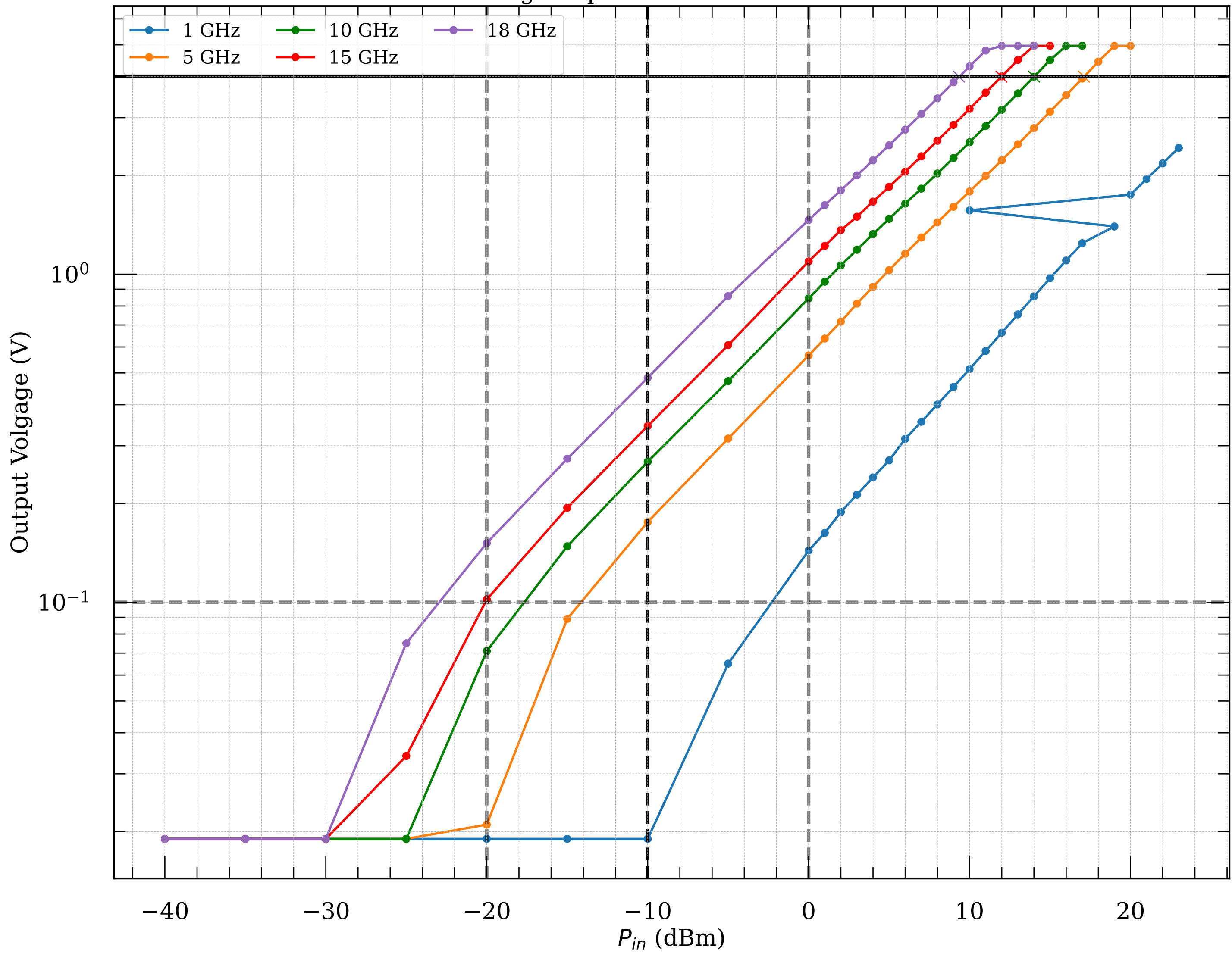
Measured voltage-to-power curve of detector module054
